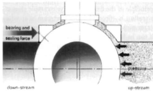
Figure 8. The sealing principle of the floating ball.
