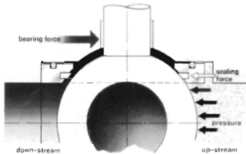
Figure 9. The sealing principle of the fixed ball.
