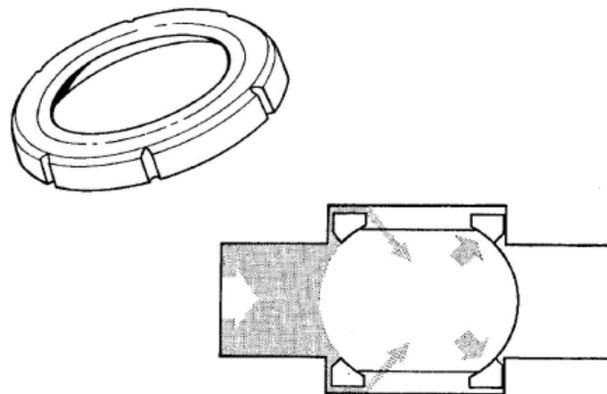
Figure 3-60. Schematic View of Ball Valve with Floating Ball and Torsion Seats, Showing Function of Pressure-Equalizing Slots in Periphery of Seats. (Courtesy of Worcestor Valve Co., Ltd.)
